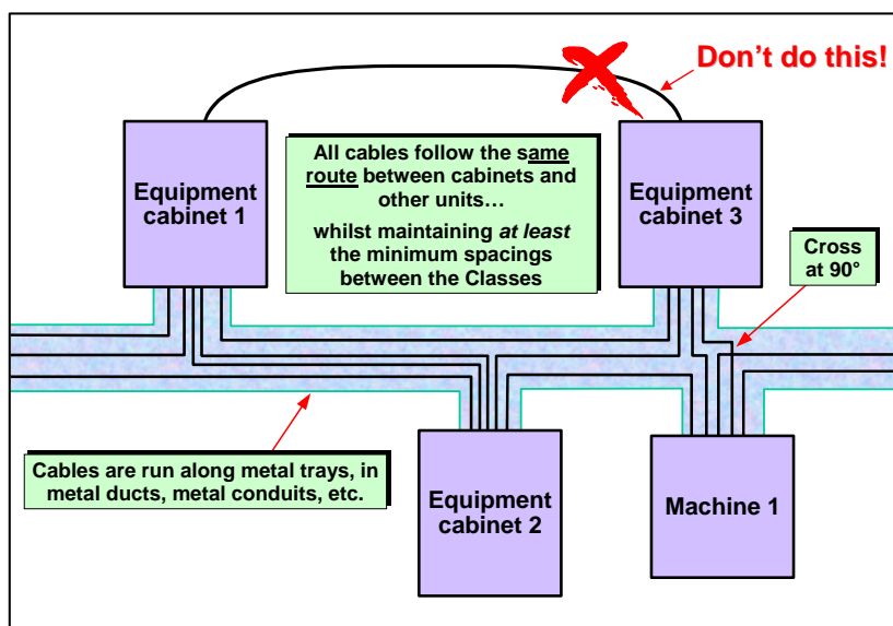
Figure 15 Routing cables along the same path whilst maintaining segregation by Class
