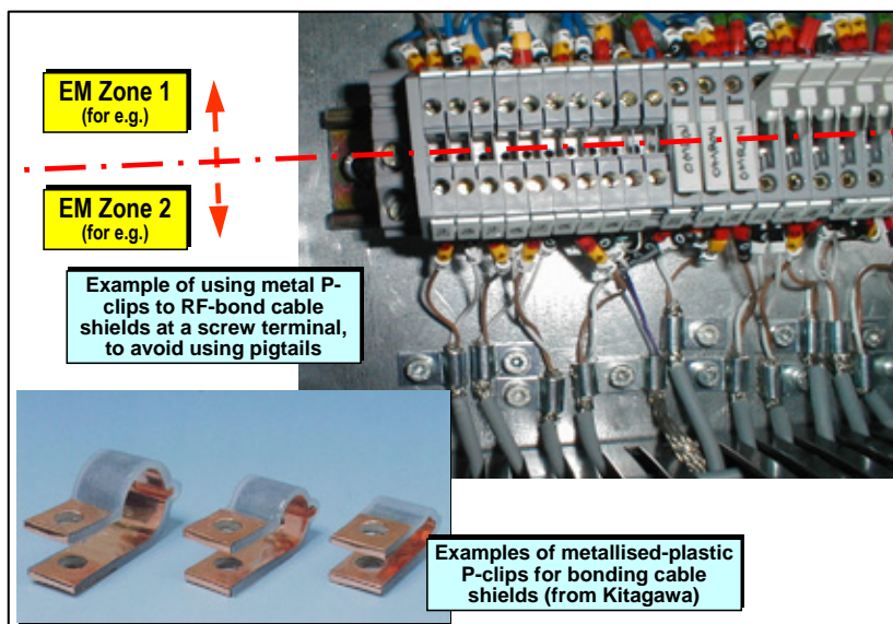
Figure 50 Example of replacing pigtails with P-clips
