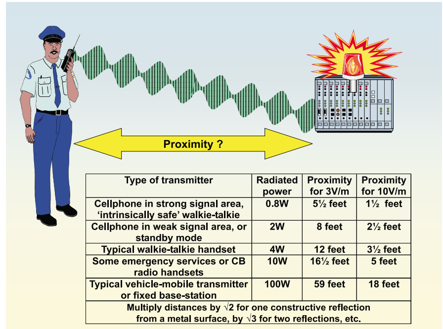
Figure 3. What do immunity standards really mean by “close proximity to a handheld radio transmitter”?
