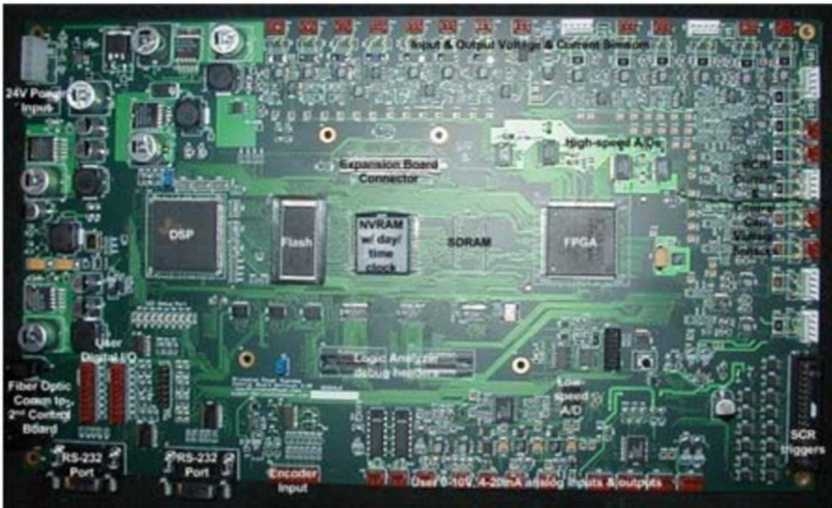
Figure 10 : Resonant Converter control board)
