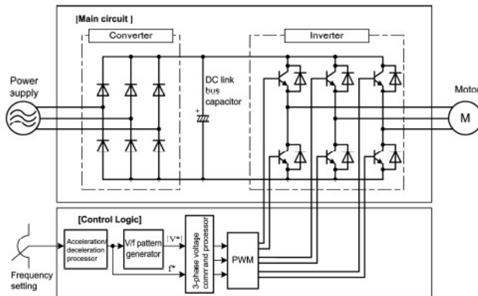
Figure 1 : Typical 6 pulse PWM VFD
