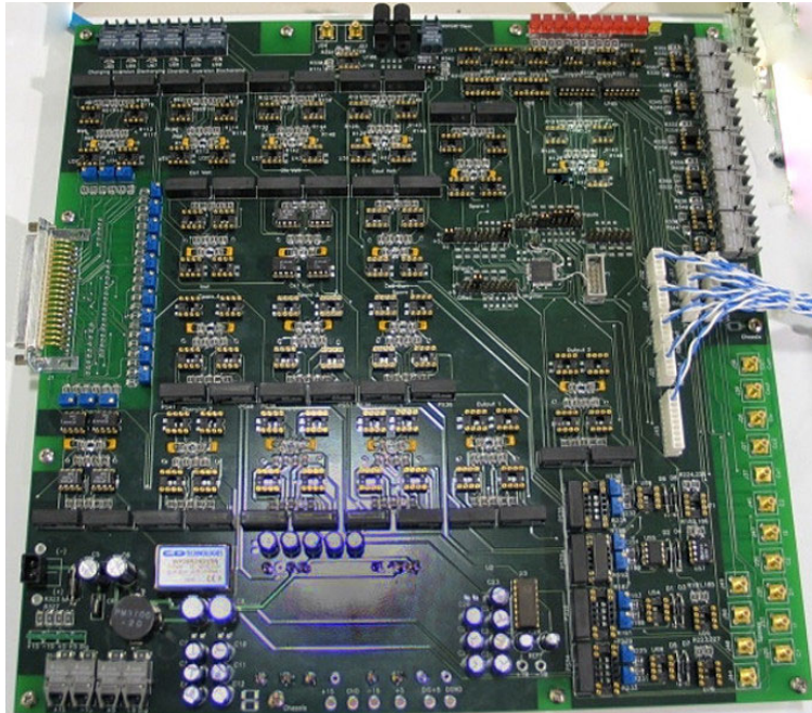
Figure 11 : Resonant Link converter instrumentation board
