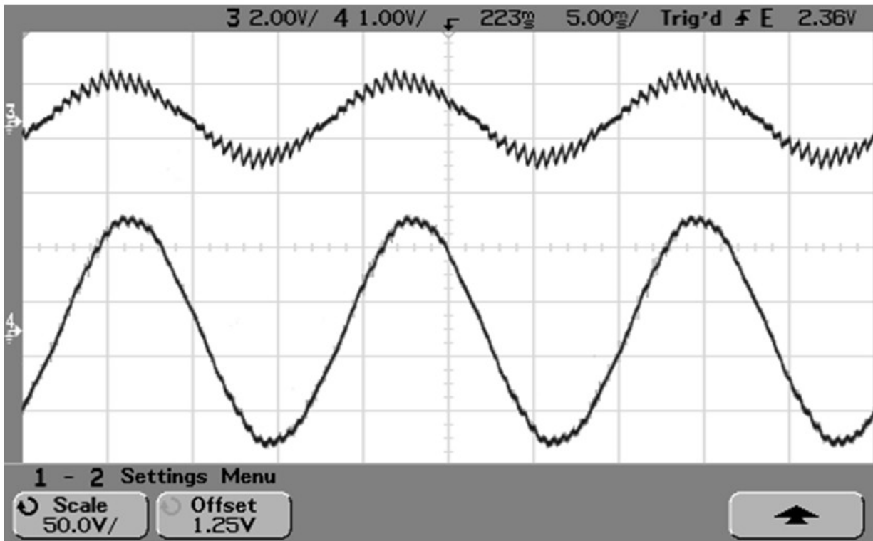
Figure 9 : Typical output voltage (top) and current (bottom) from 250kW Resonant Link ESP converter. du/dt recorded was 1.2V/microsecs. Both converter outputs were unfiltered.
