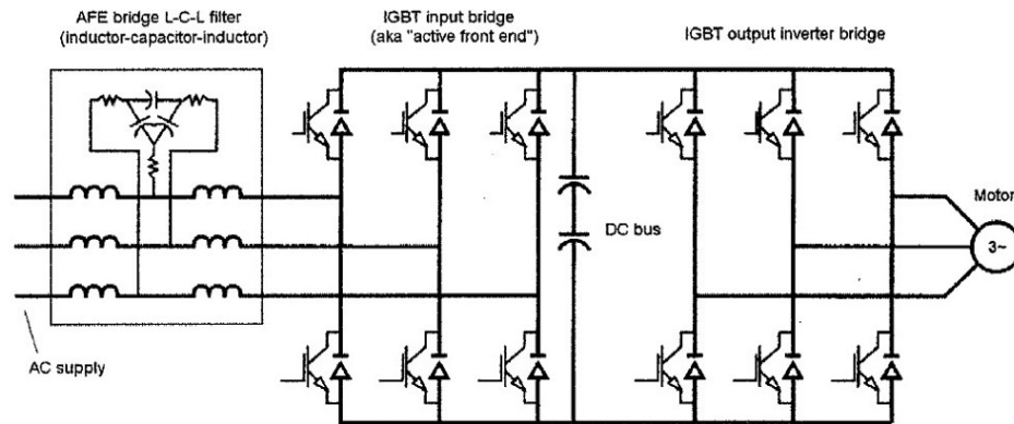
Figure 2 : Typical simplified schematic of AFE VFD
