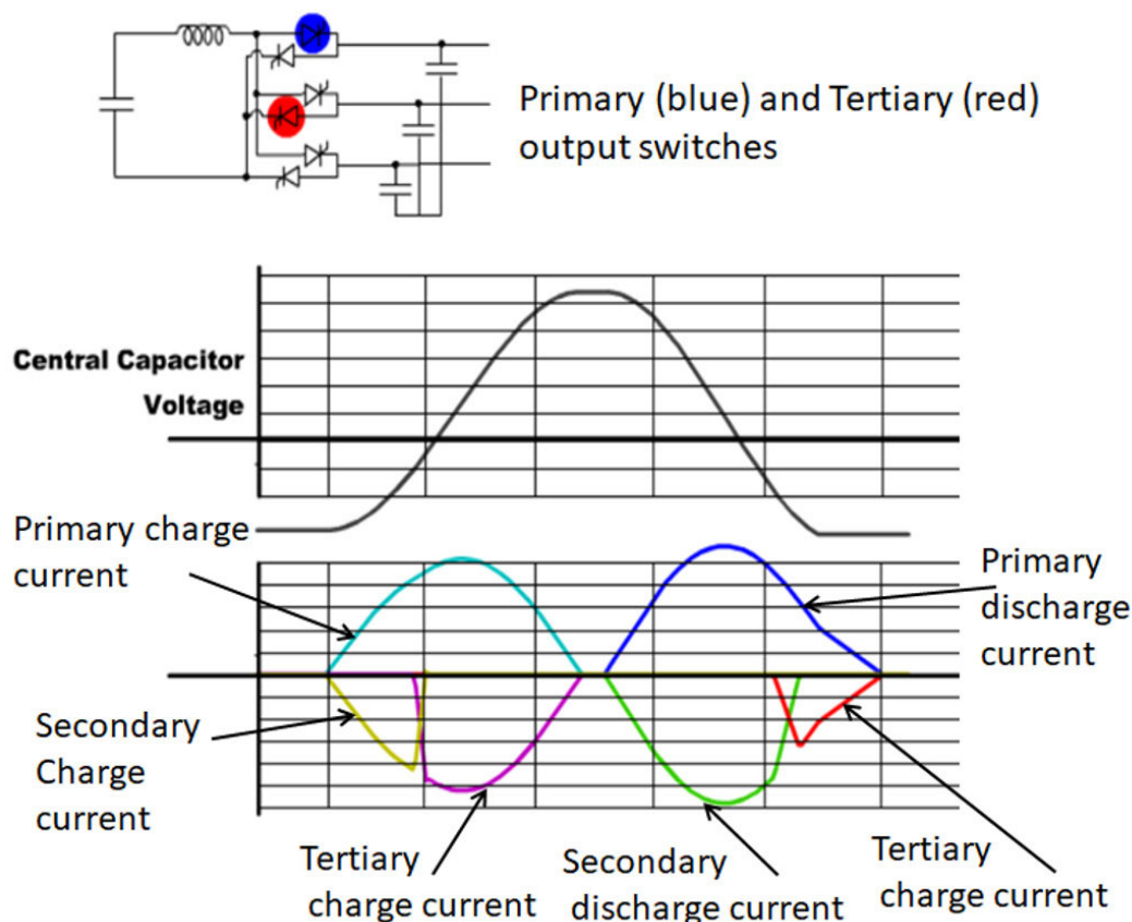
Figure 7 : Resonant Link converter charge and discharge operation
