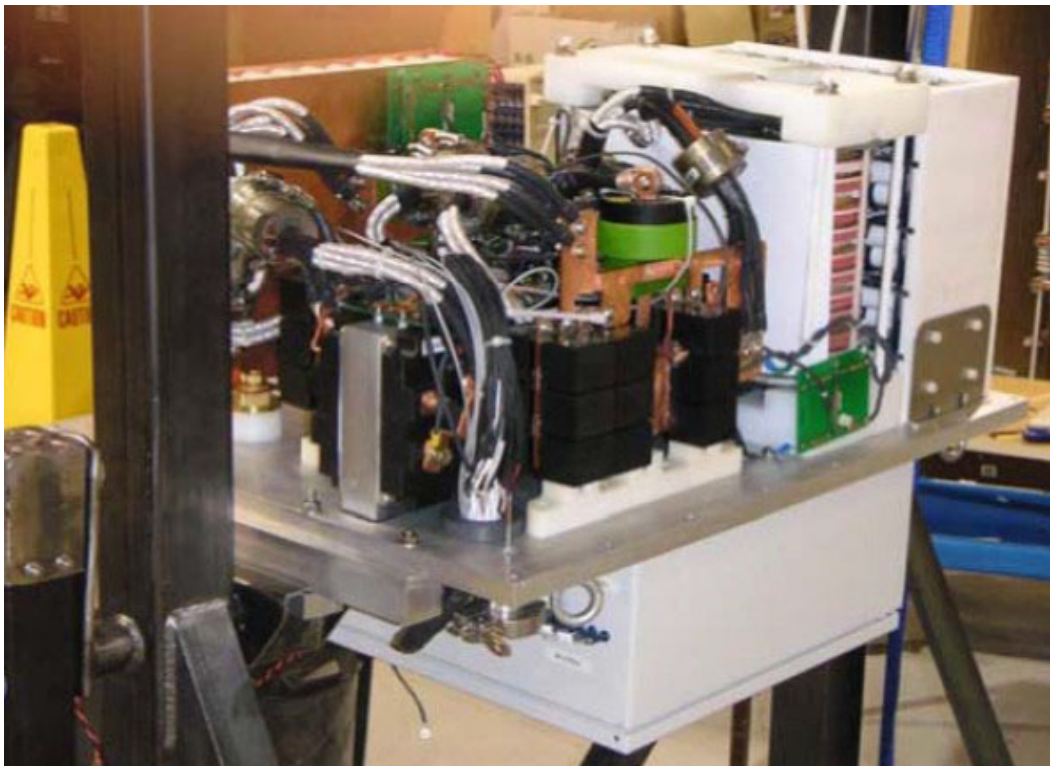
Figure 5 : Example of 250kW Resonant Link converter (3 x 480V in/50kVDC out). 11kg, 250kVA nanocrystalline transformer mounted below. Military application.
