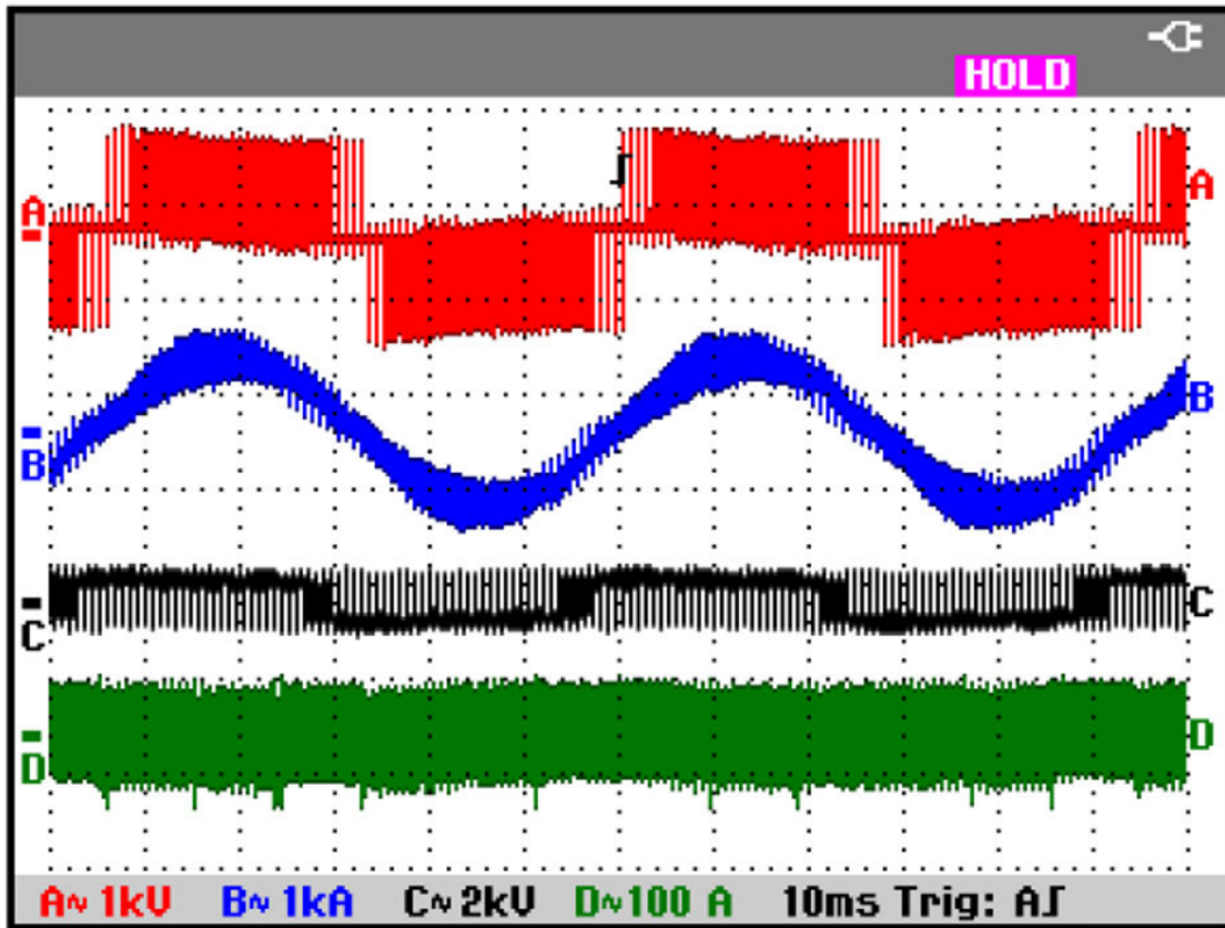
Figure 3 : A = line voltage. B = phase current. C = common mode voltage. D = common mode current.
