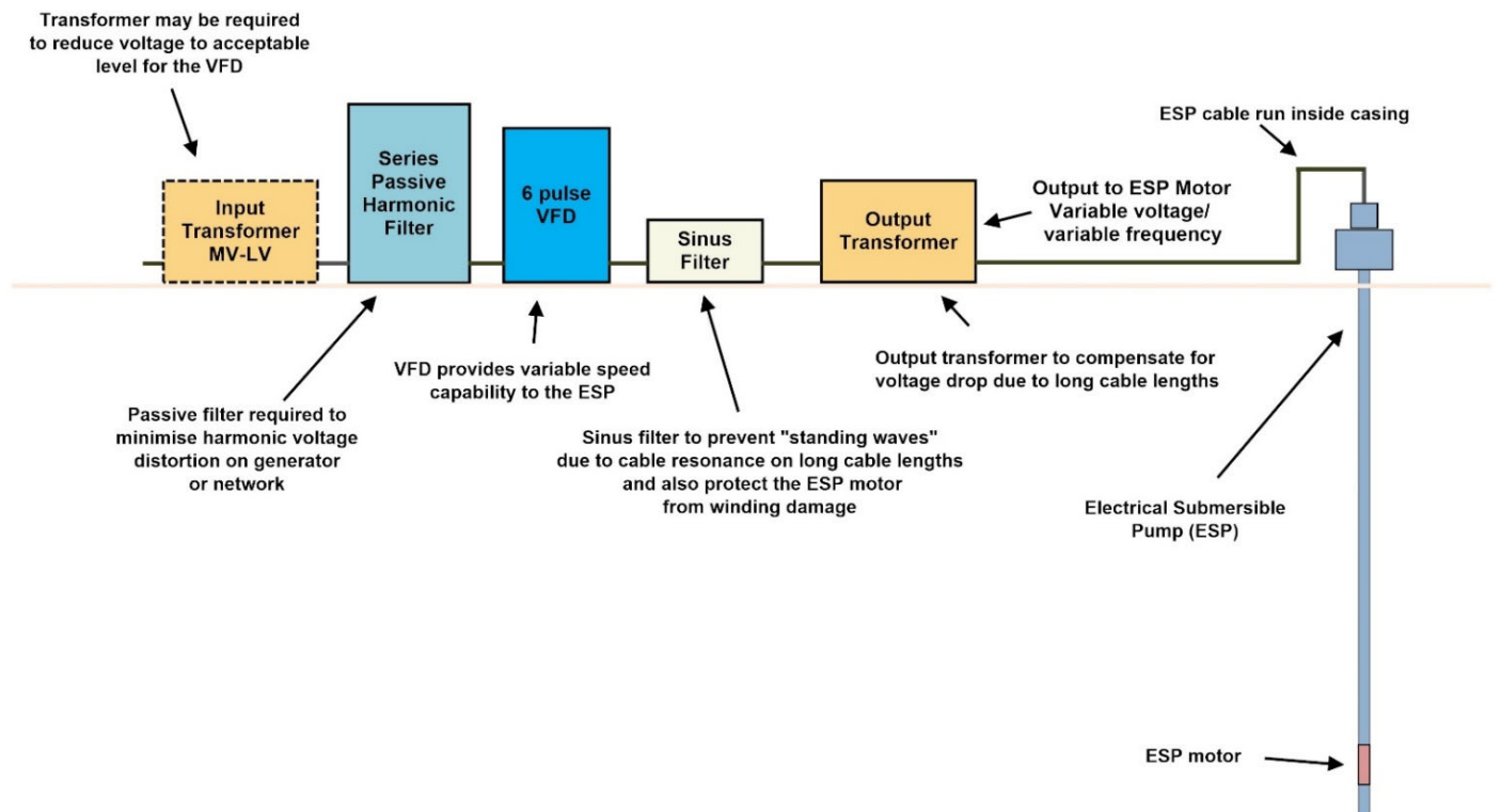
Figure 4 : Typical drive train for low voltage 6 pulse ESP PWM VFD
