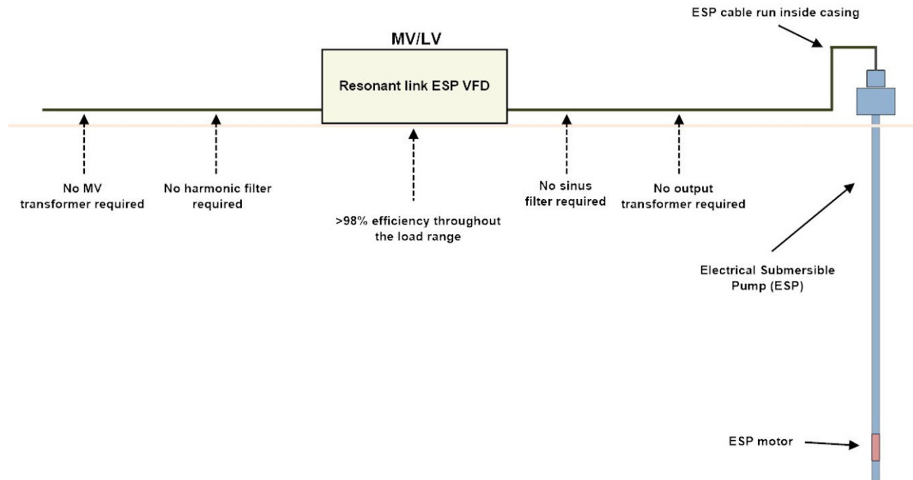
Figure 6 : No additional equipment required for Resonant Link converter for ESP VFD applications
