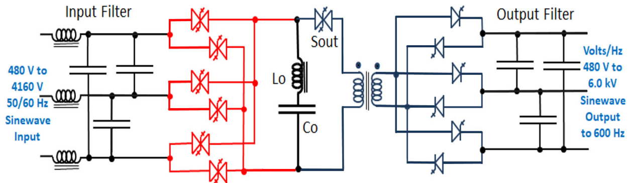
Figure 7 : Single module LV/MV Resonant Link ESP converter with step-up/step down
