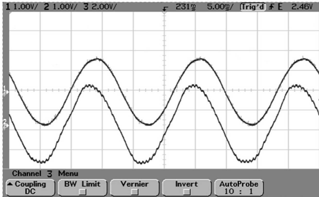
Figure 8 : Typical input voltage (top) and current (bottom) of 250kW Resonant Link converter. THDi < 1%. Unity displacement power factor.
