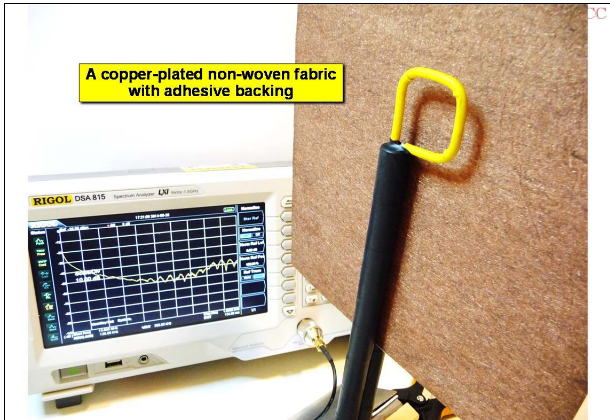
Figure 65 A copper-plated non-woven fabric with adhesive backing
