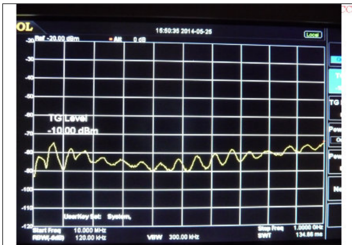
Figure 15 Looking for shield imperfections with two CF probes – the display (1)
