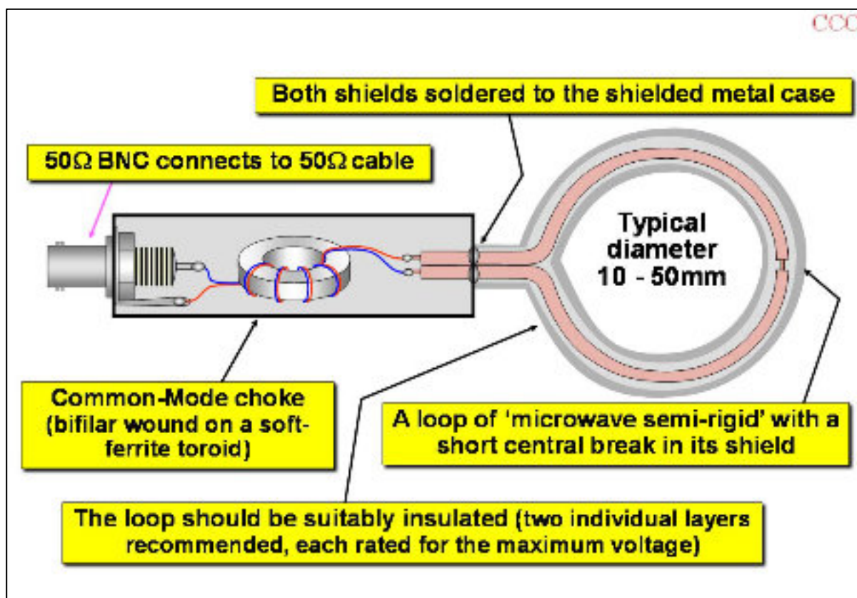
Figure 1 The construction of a good-quality close-field magnetic probe
