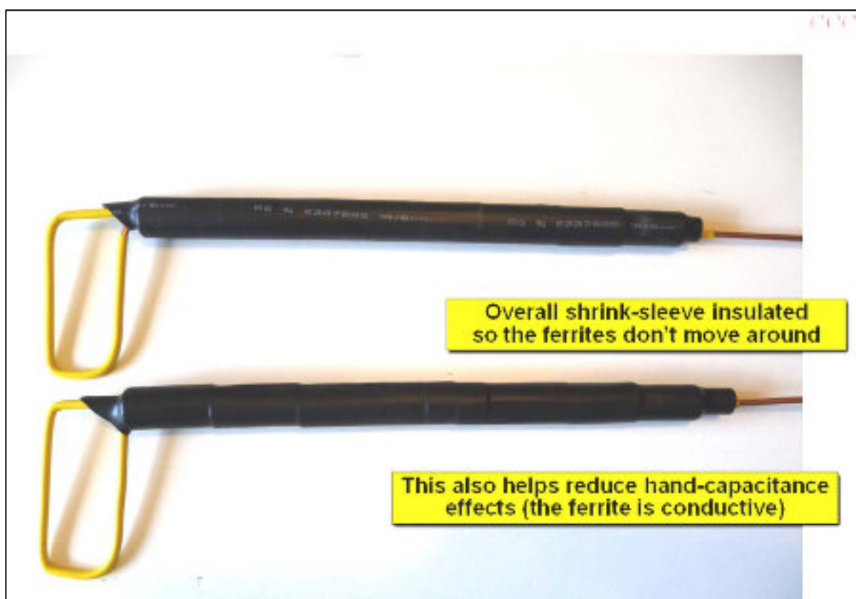
Figure 13 My new RG405 probes when finally assembled
