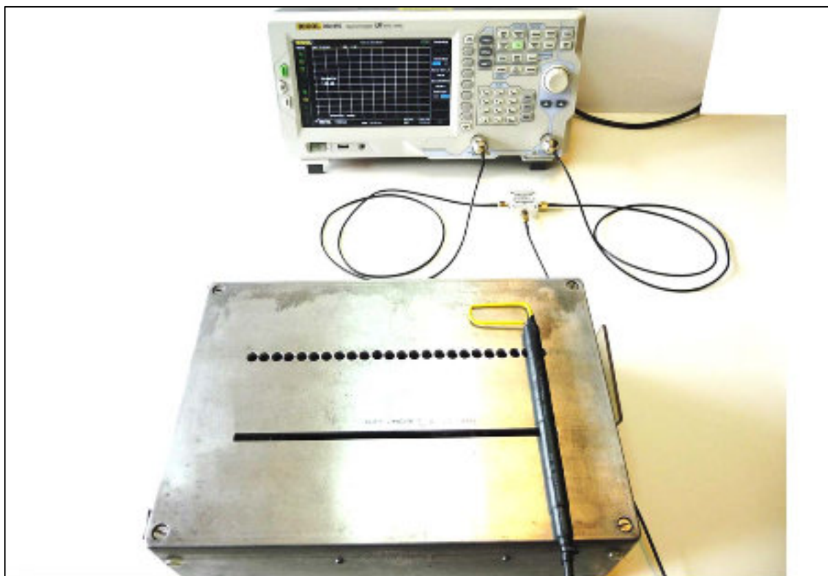
Figure 28 Looking for shielding imperfections with a reflectometer – normalising
