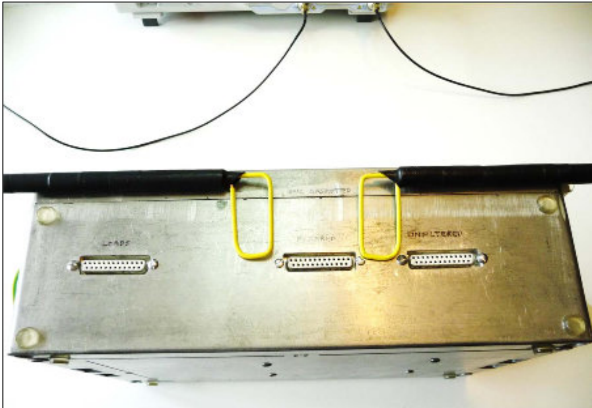
Figure 24 Looking for gasketting imperfections with two CF probes – the set-up (6)
