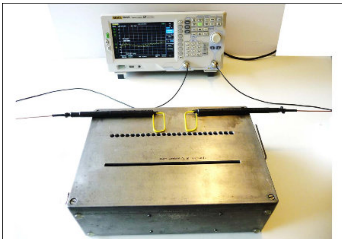
Figure 14 Looking for shield imperfections with two CF probes – the set-up (1)
