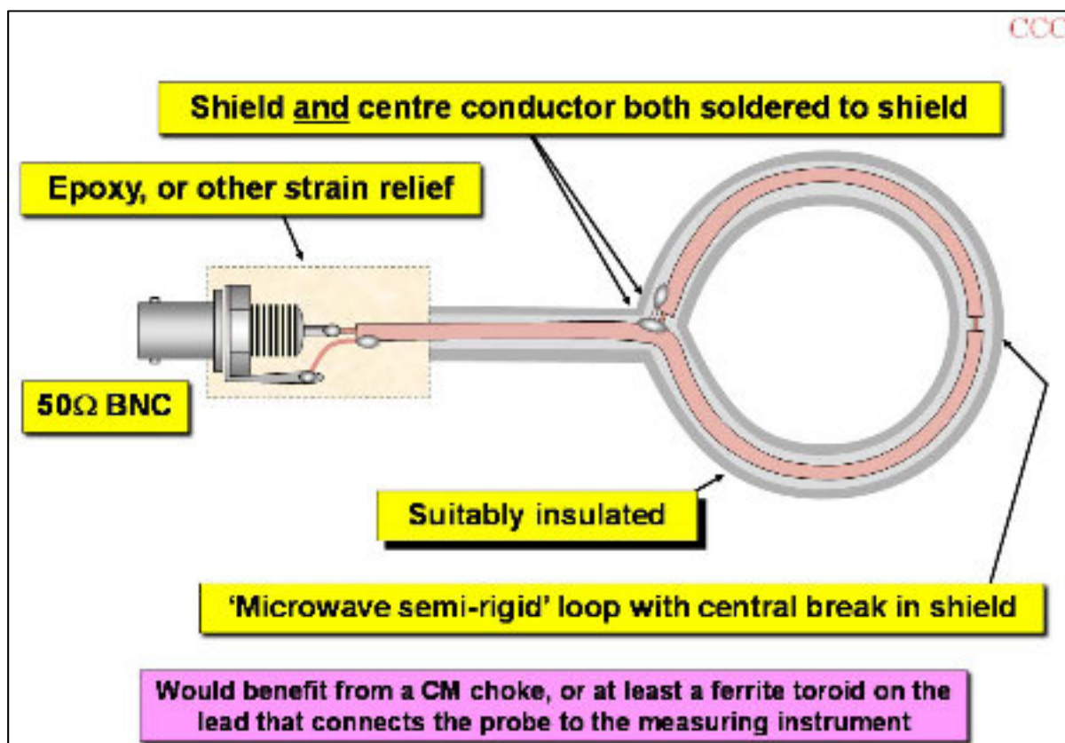
Figure 2 An easier magnetic field close-field probe design (but not so good)
