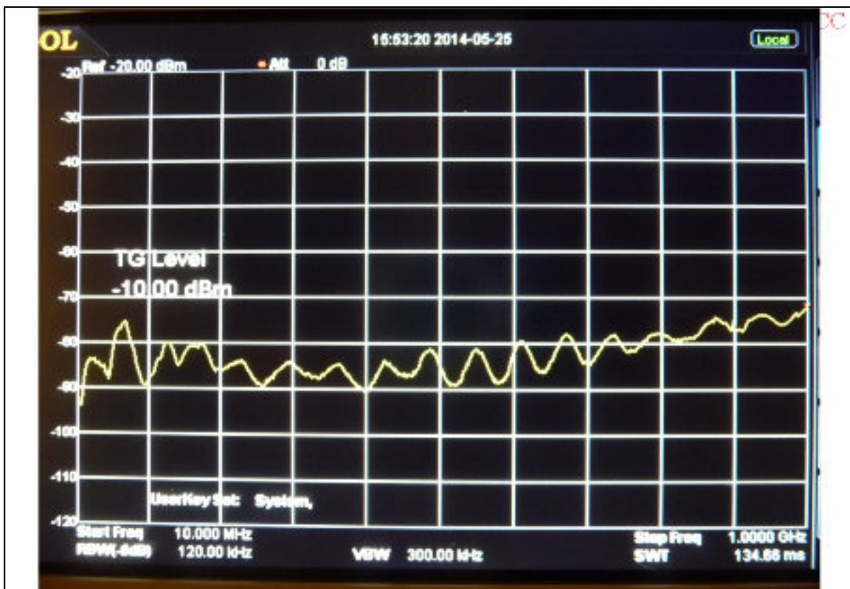
Figure 17 Looking for shield imperfections with two CF probes – the display (2)
