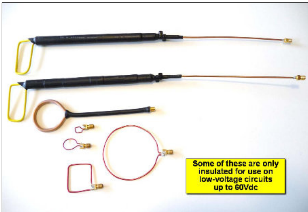
Figure 5 The range of close-field probes that I use (at the time of writing)
