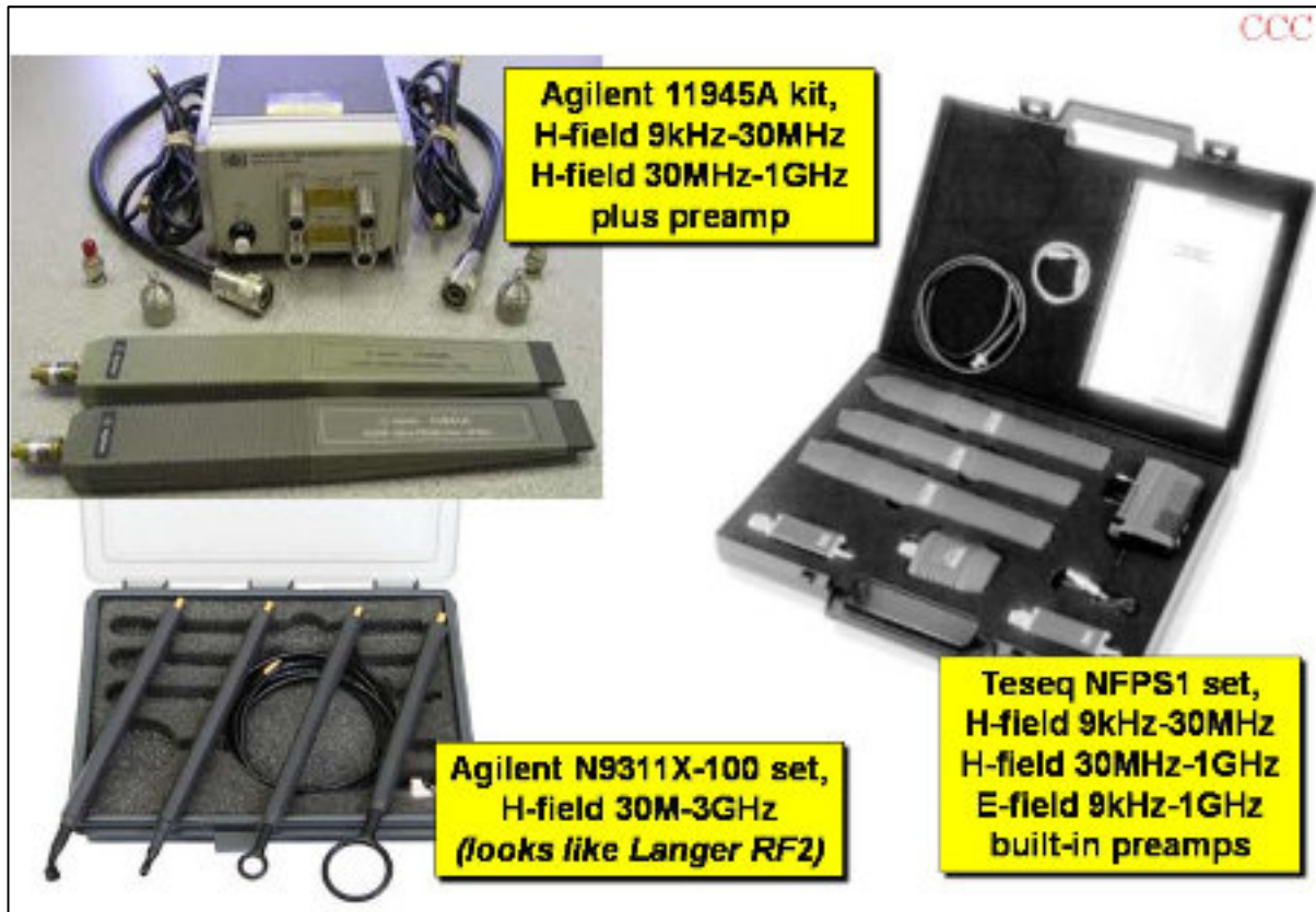
Figure 8 Hewlett-Packard's venerable close-field probes, and currently available ones from Agilent (soon to be renamed Keysight Technologies) and Teseq (which used to be Chase EMC)
