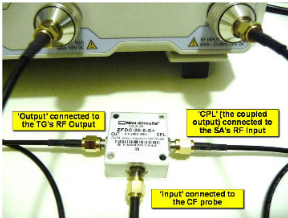
Figure 29 A closer view of the directional coupler in Figure 28
