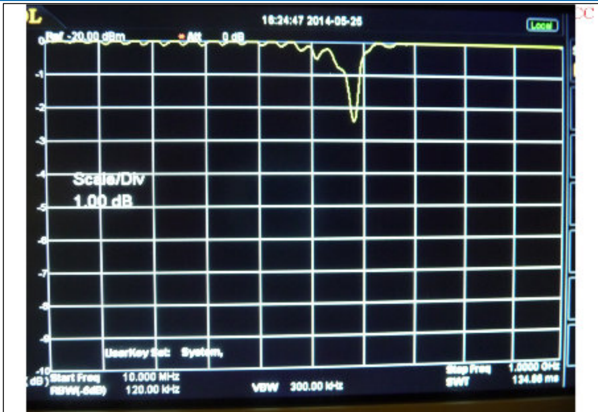
Figure 34 Looking for shielding imperfections with a reflectometer – the display (9)
