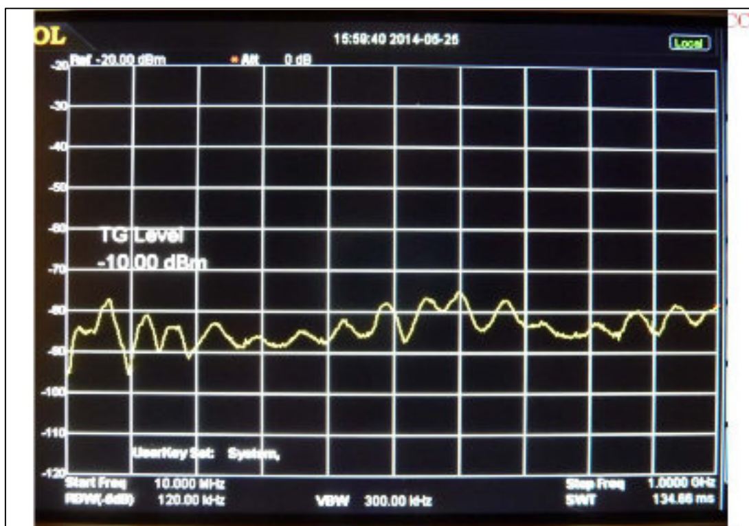
Figure 23 Looking for shield imperfections with two CF probes – the display (5)
